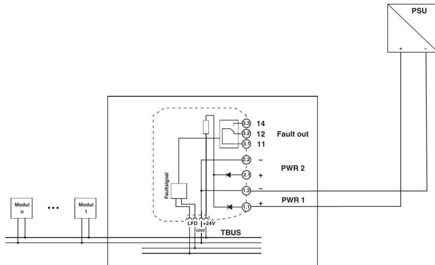
Figure 5-3 Supply by means of one power supply
